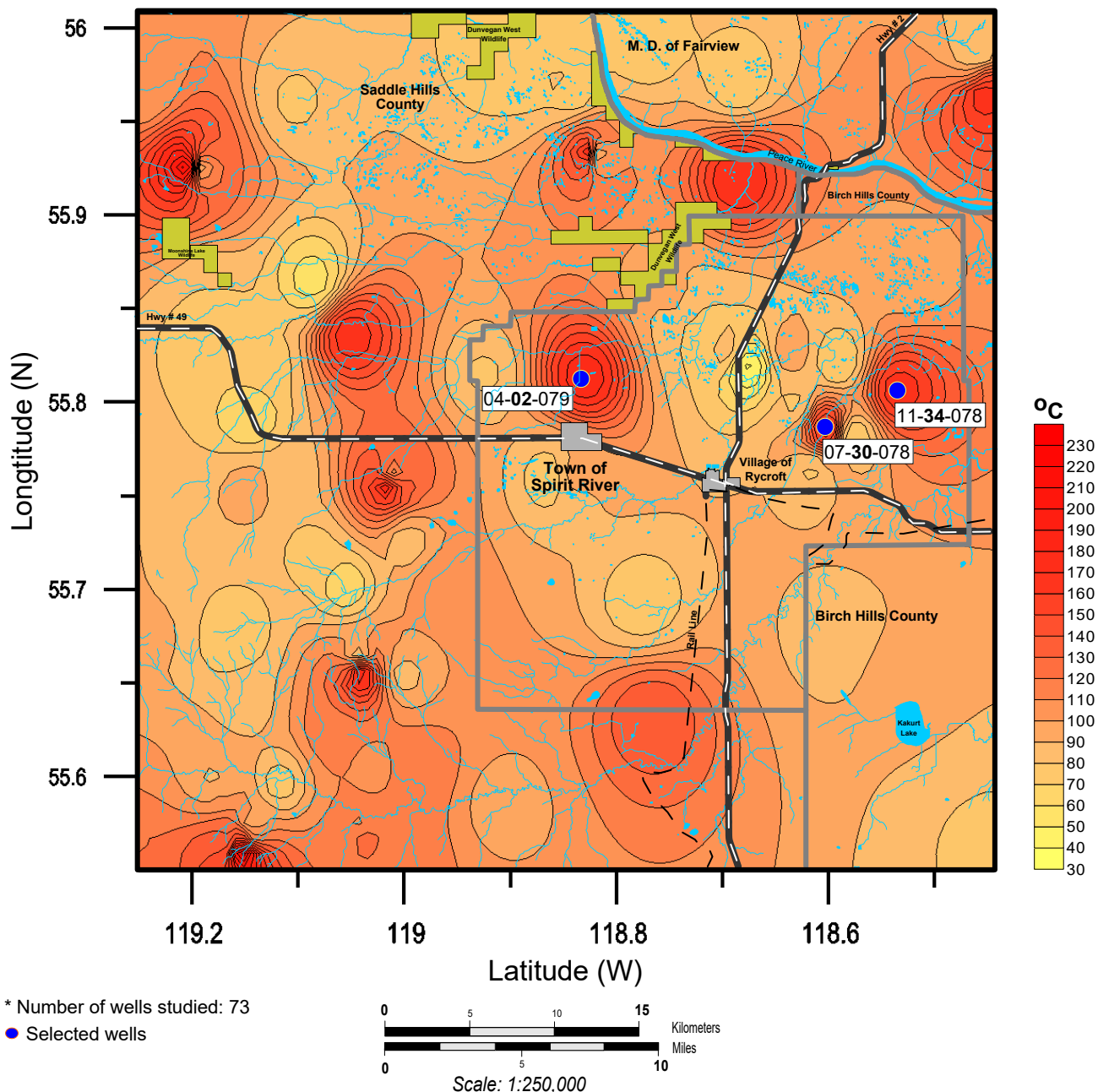
Corrected Bottom-Hole Temperature Map (at Depths Greater than 2.3km - M. D. of Spirit River)
