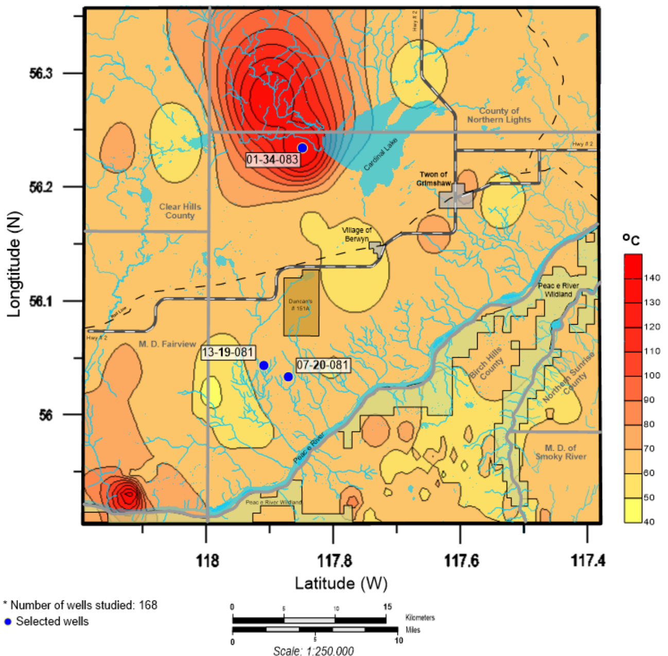
Corrected Bottom-Hole Temperature Map (at Depths Greater than 1.8km - M. D. of Peace)
