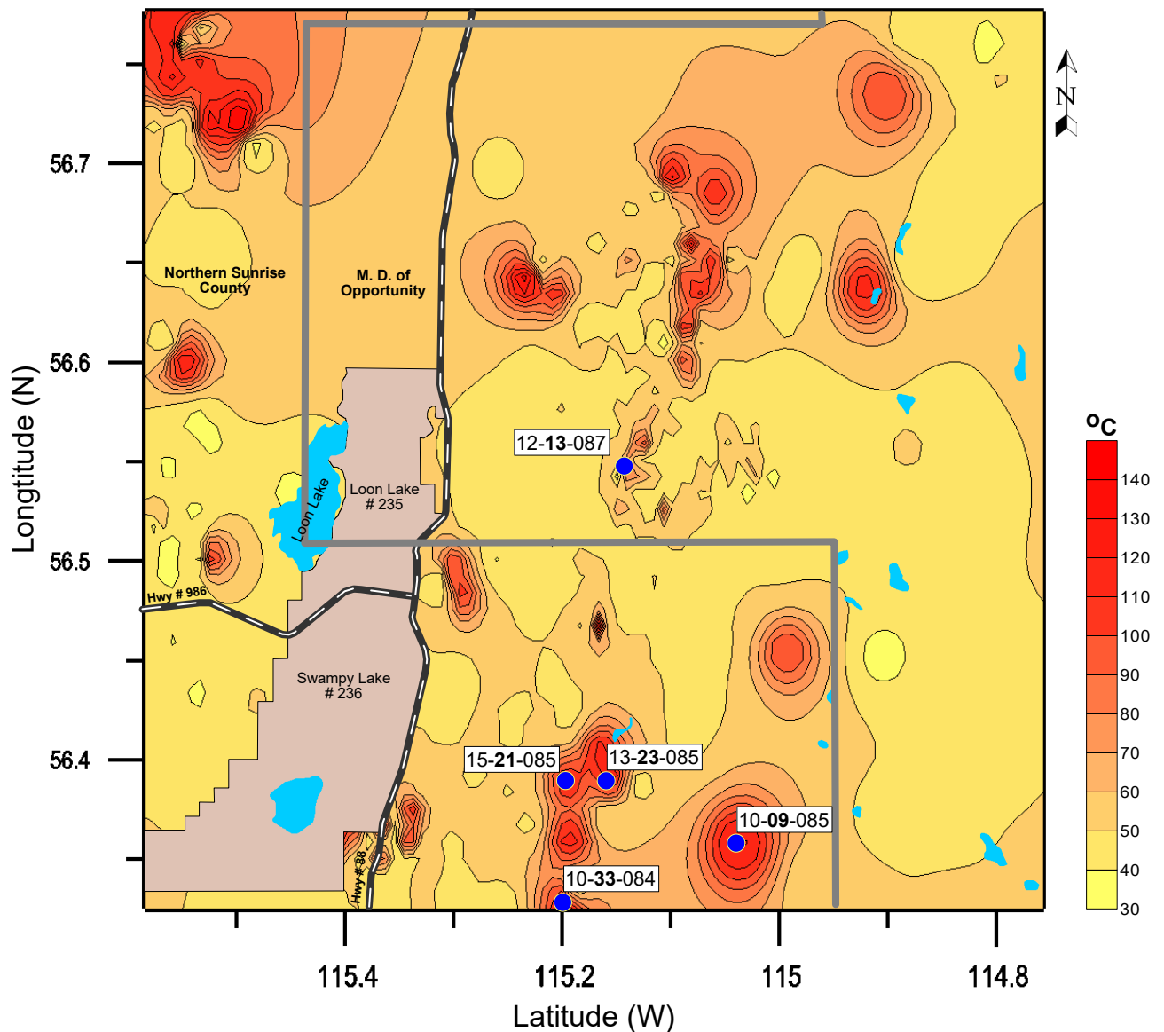
Corrected Bottom-Hole Temperature Map (at Depths Greater than 1.5km - M. D. of Opportunity)
