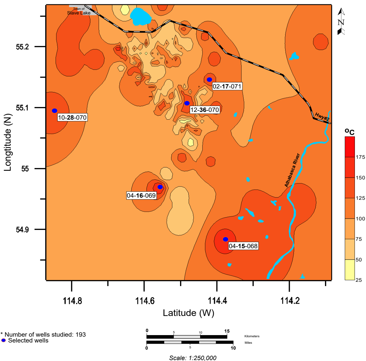
Corrected Bottom-Hole Temperature Map (at Depths Less than 1.8km - M.D. of Lesser Slave River)
