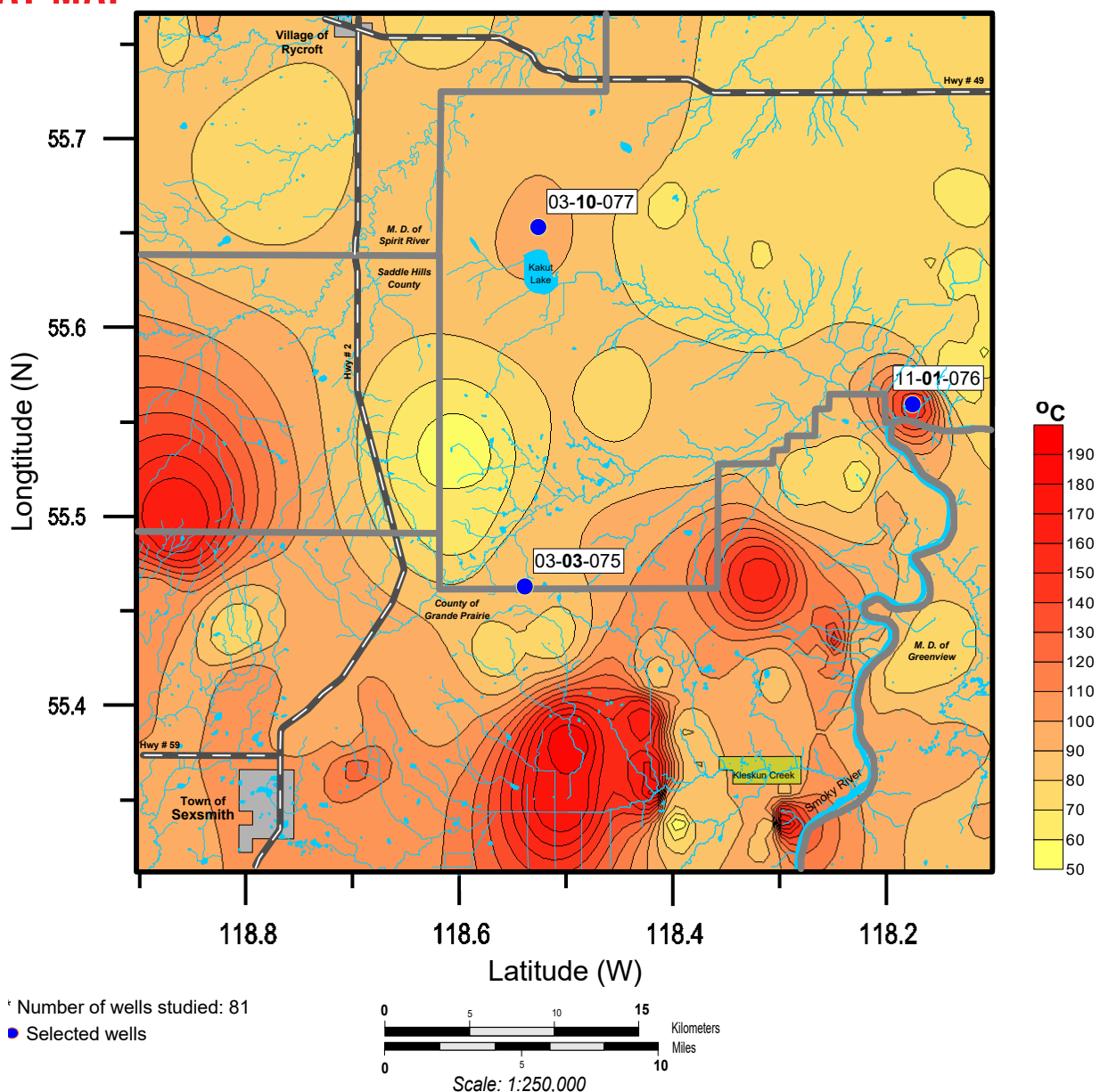
Corrected Bottom-Hole Temperature Map (at Depths Greater than 2.4km - Birch Hills County)
