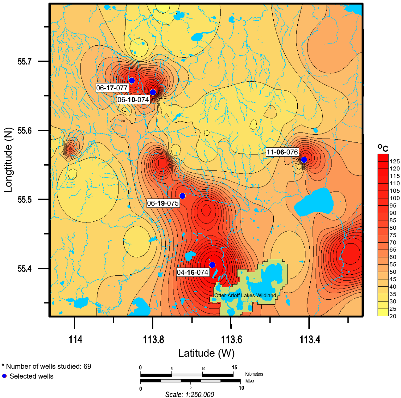
Corrected Bottom-Hole Temperature Map (at Depths Greater than 0.8km - Wabasca South)
