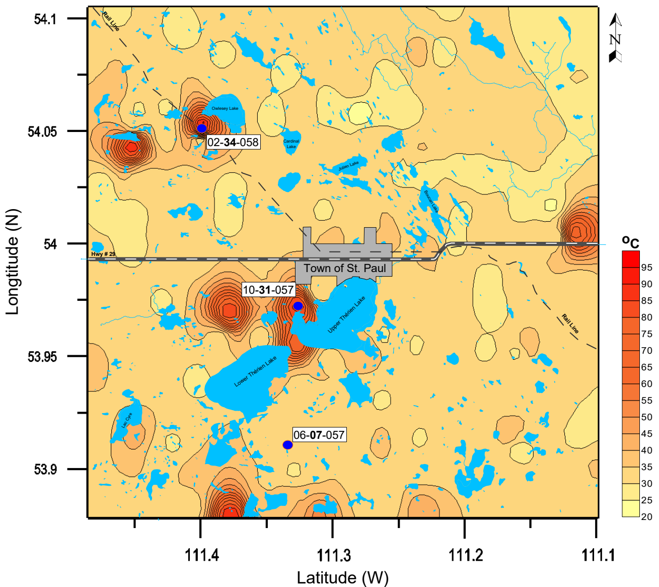
Corrected Bottom-Hole Temperature Map (at Depths Greater than 0.6km - Town of St. Paul)
