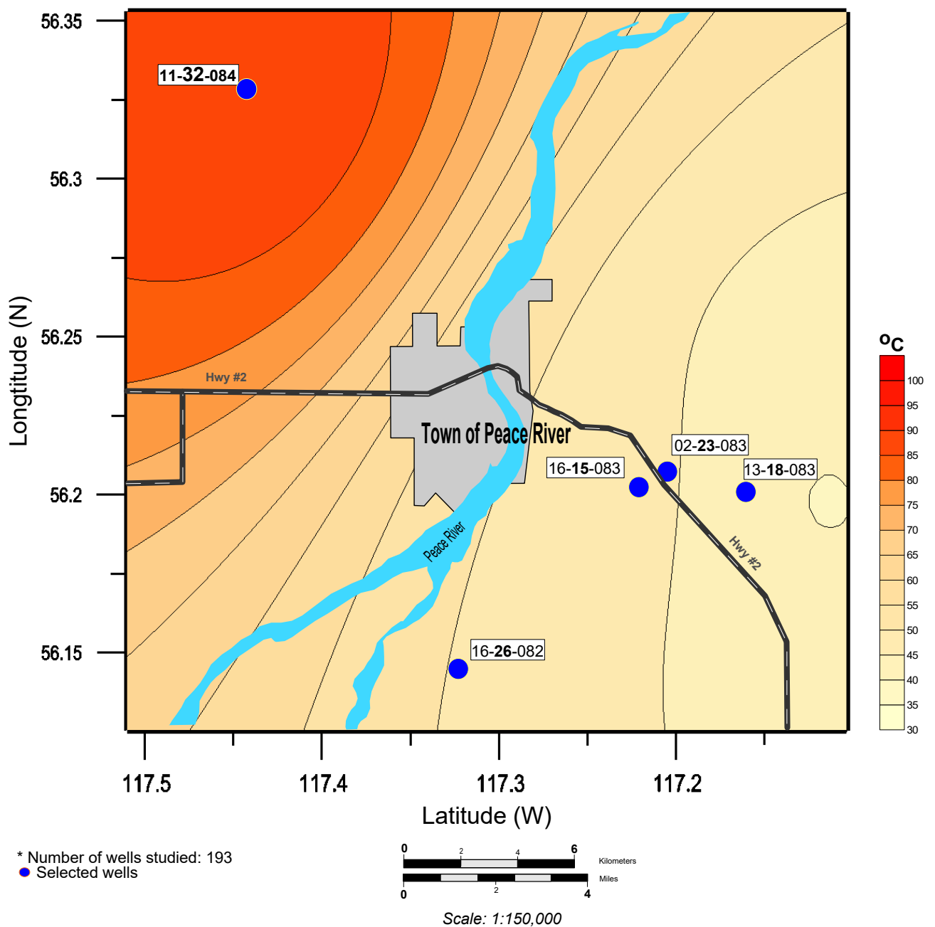
Corrected Bottom-Hole Temperature Map (at Depths Greater than 1km - Town of Peace River)
