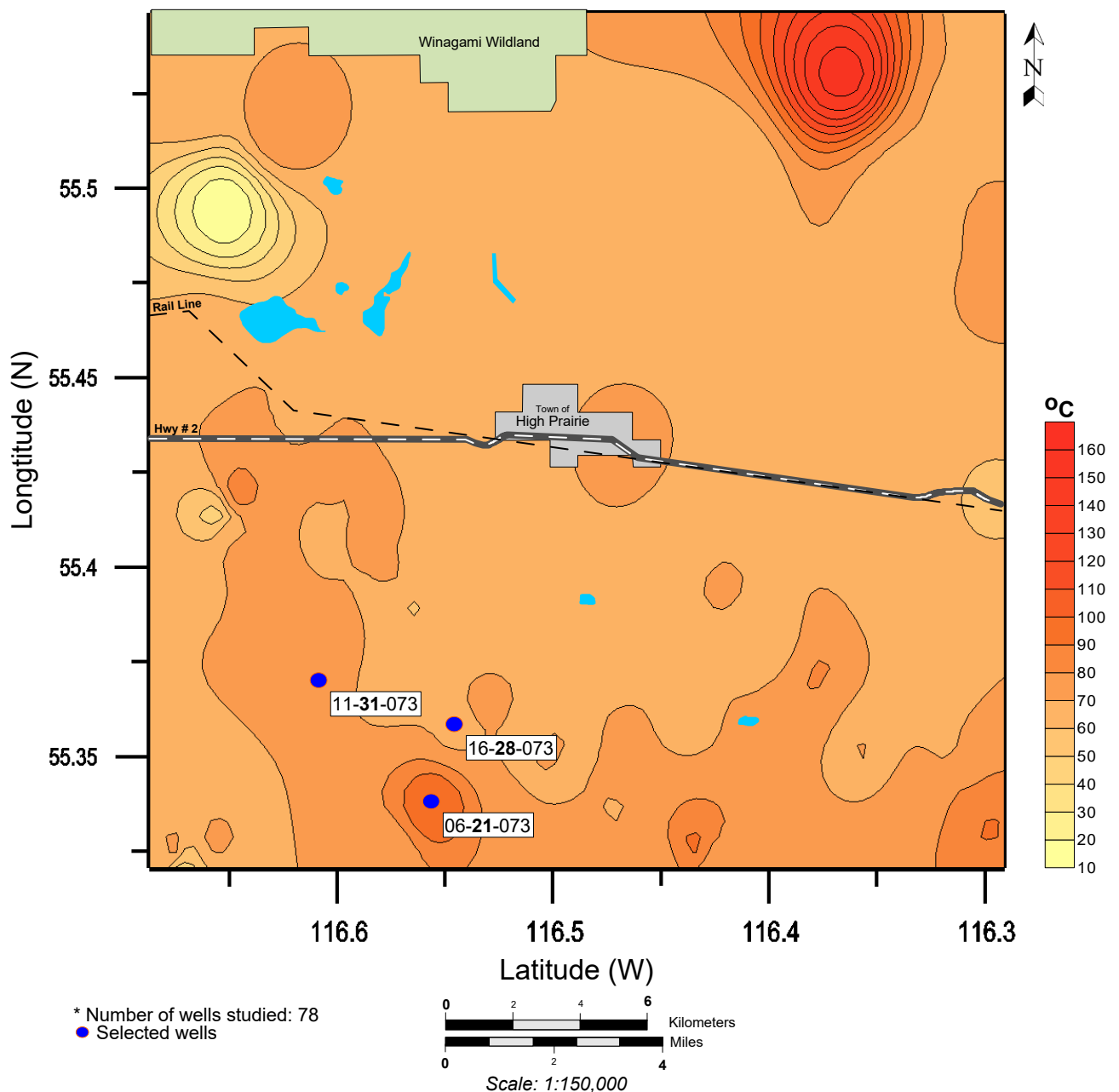
Corrected Bottom-Hole Temperature Map (at Depths Greater than 2 km - Town of High Prairie)
