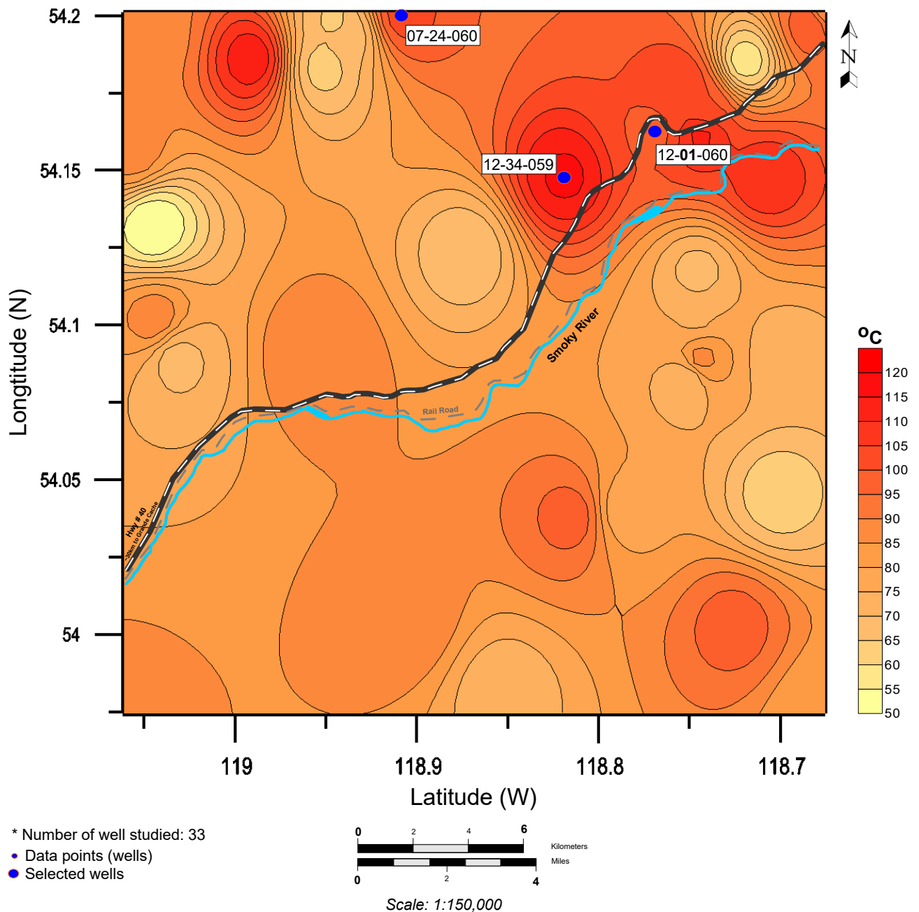
Corrected Bottom-Hole Temperature Map (at Depths Greater than 2.5km - 15km NW of Town of Grande Cache)
